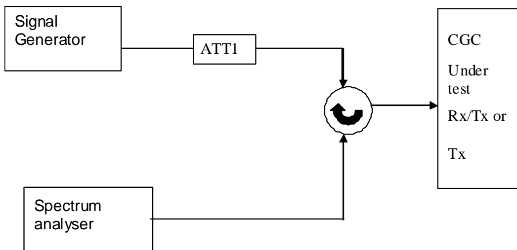
Figure D.3: Measuring system Set-up for CGC Transmit Intermodulation Tests
